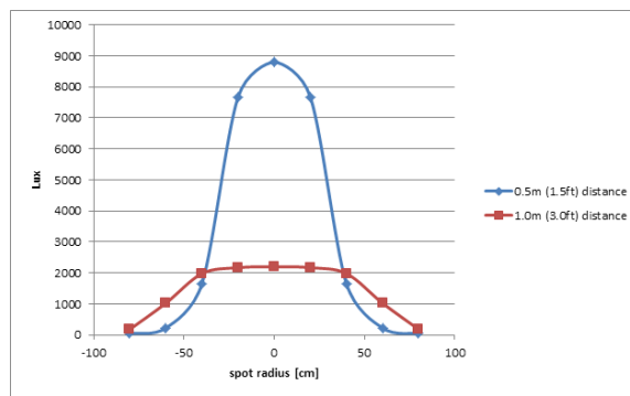
Light Output AOS-LED W40 500mm / 1000mm distance
