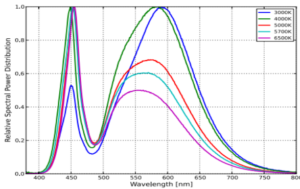
LED Spectral Range (curve: 5700K)
