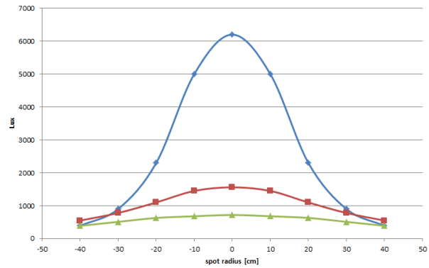
Light Output AOS-LED W15 250mm / 500mm / 750mm distance
