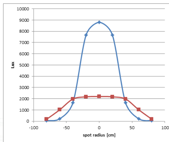
Light Output A-LED W40 500mm / 1000mm distance
