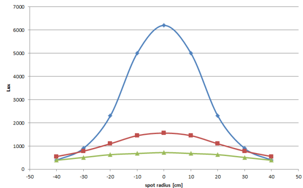
Light Output A-LED W15 250mm / 500mm / 750mm distance
